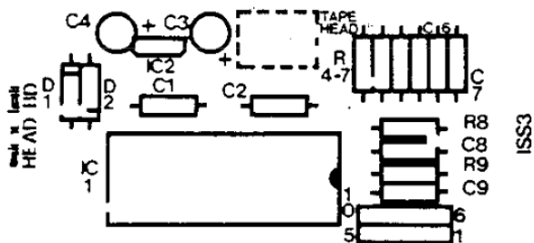
ZX Microdrive Head Board Layout
