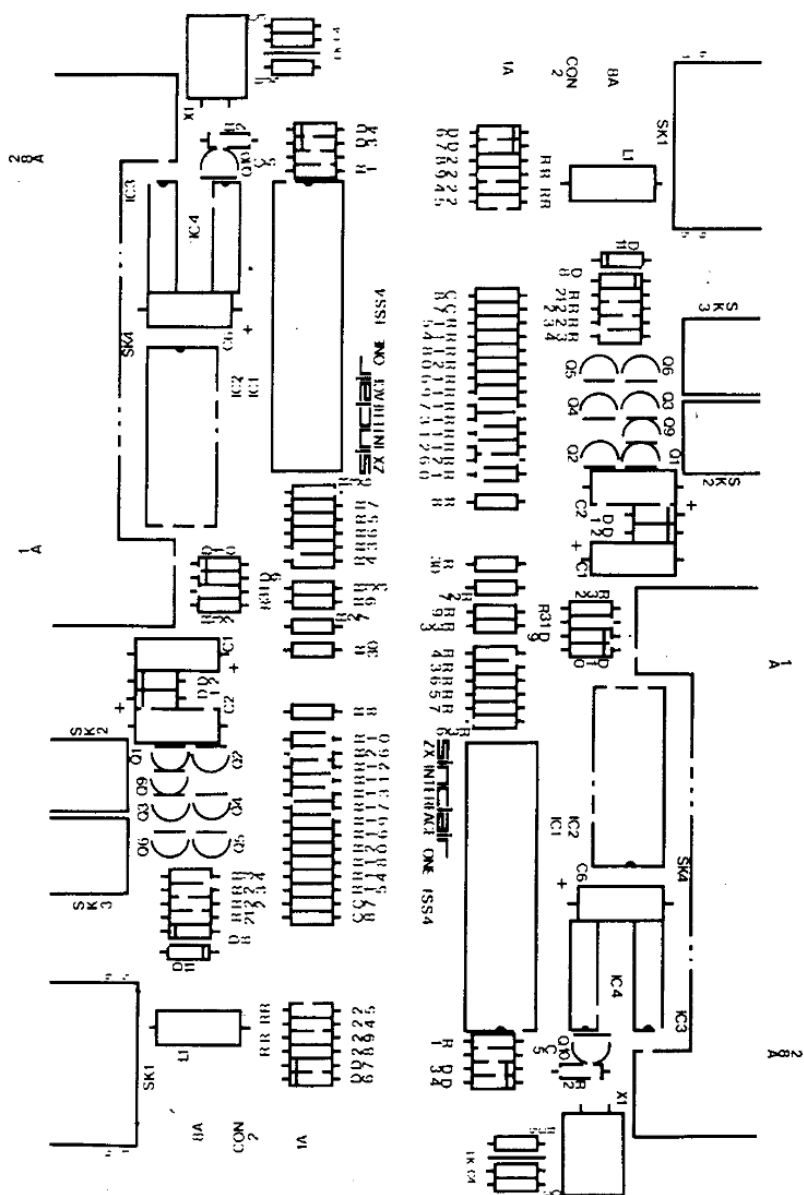
ZX Interface 1 Board Layout
