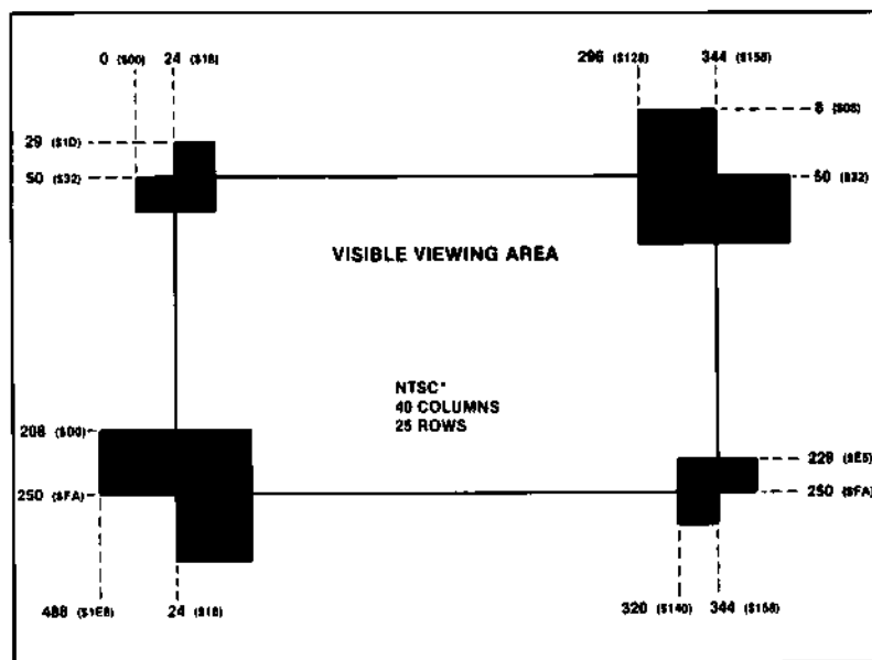
Figure 6-7. Visible Sprite Coordinates
